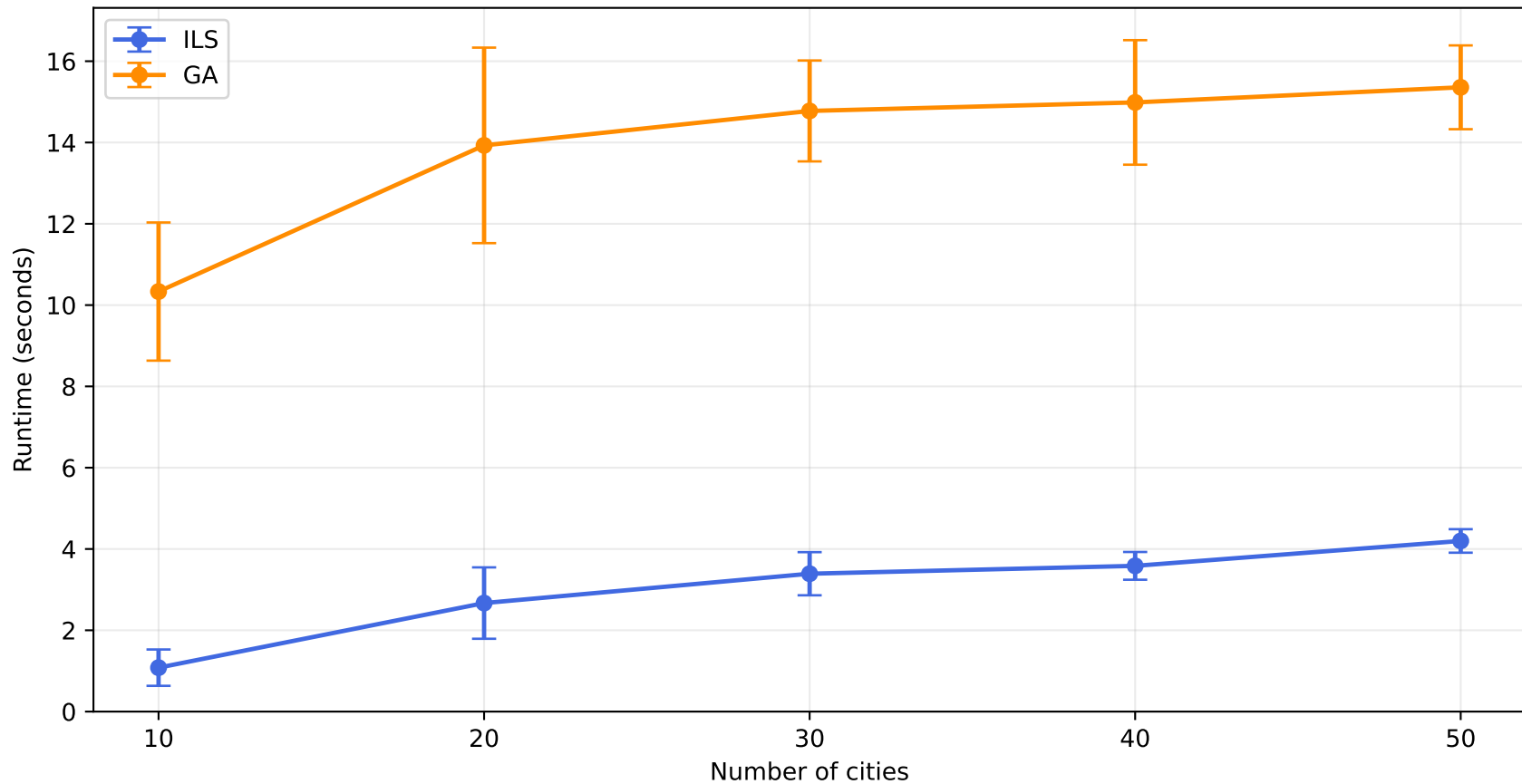
Runtime — Mean \pm 1 SD Across 10 Runs
