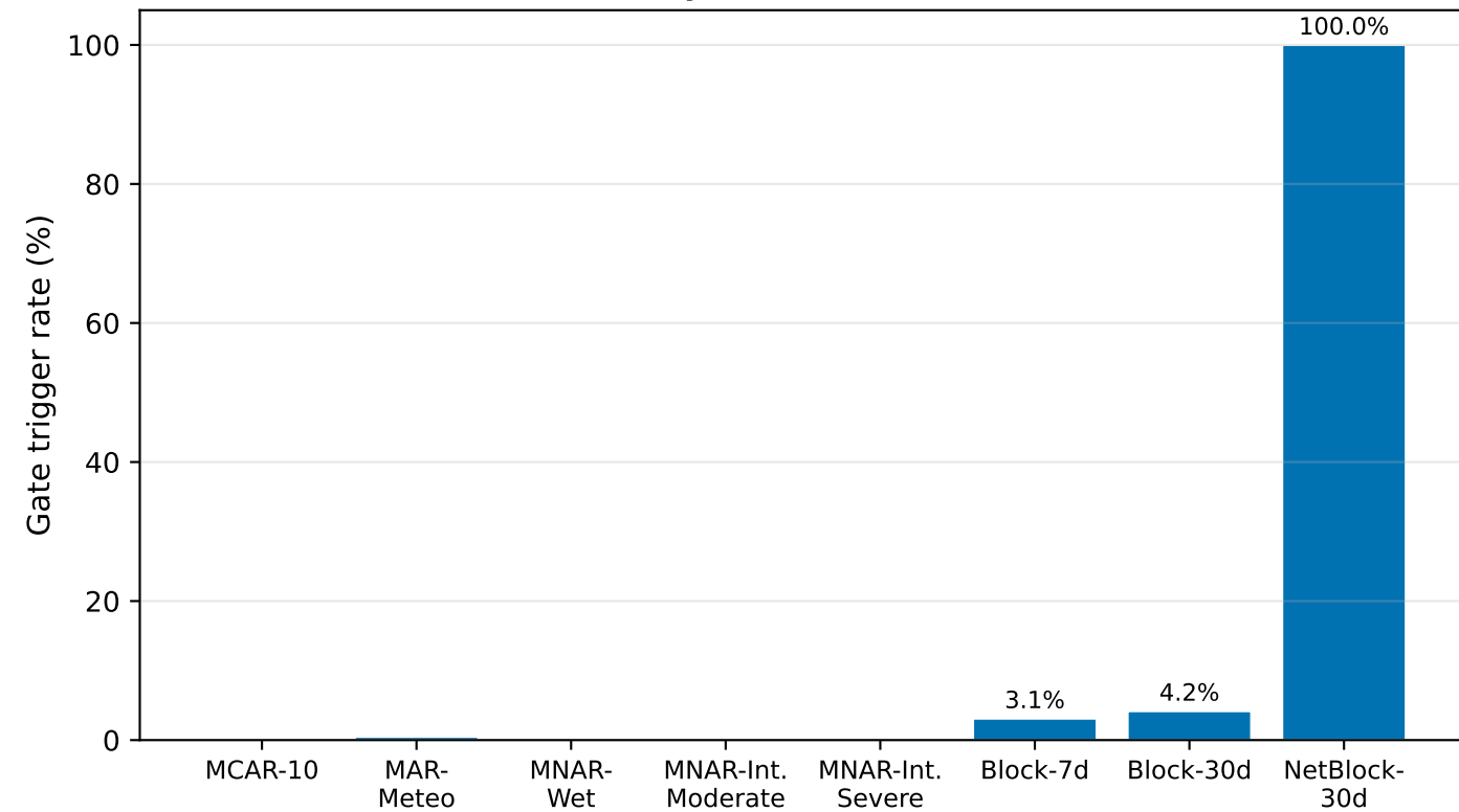
(b) Selectivity: how often the gate actually routes to fallback
