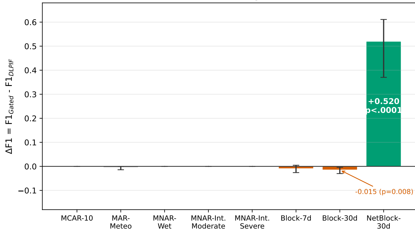
(a) Recovery vs preservation (seed=42 bootstrap 95% CI)
