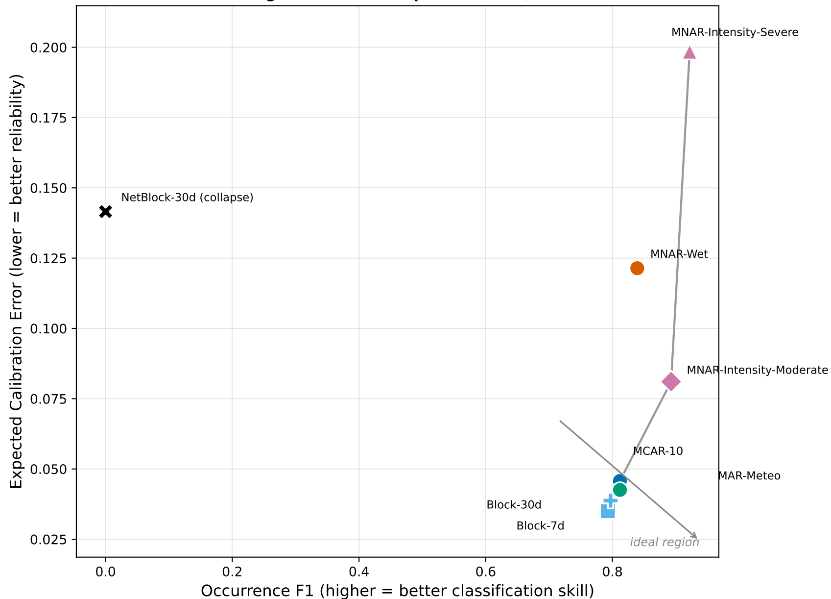
Apparent classification skill vs probabilistic reliability (Platt-calibrated Stage-1 occurrence probabilities, mean over 3 seeds)
