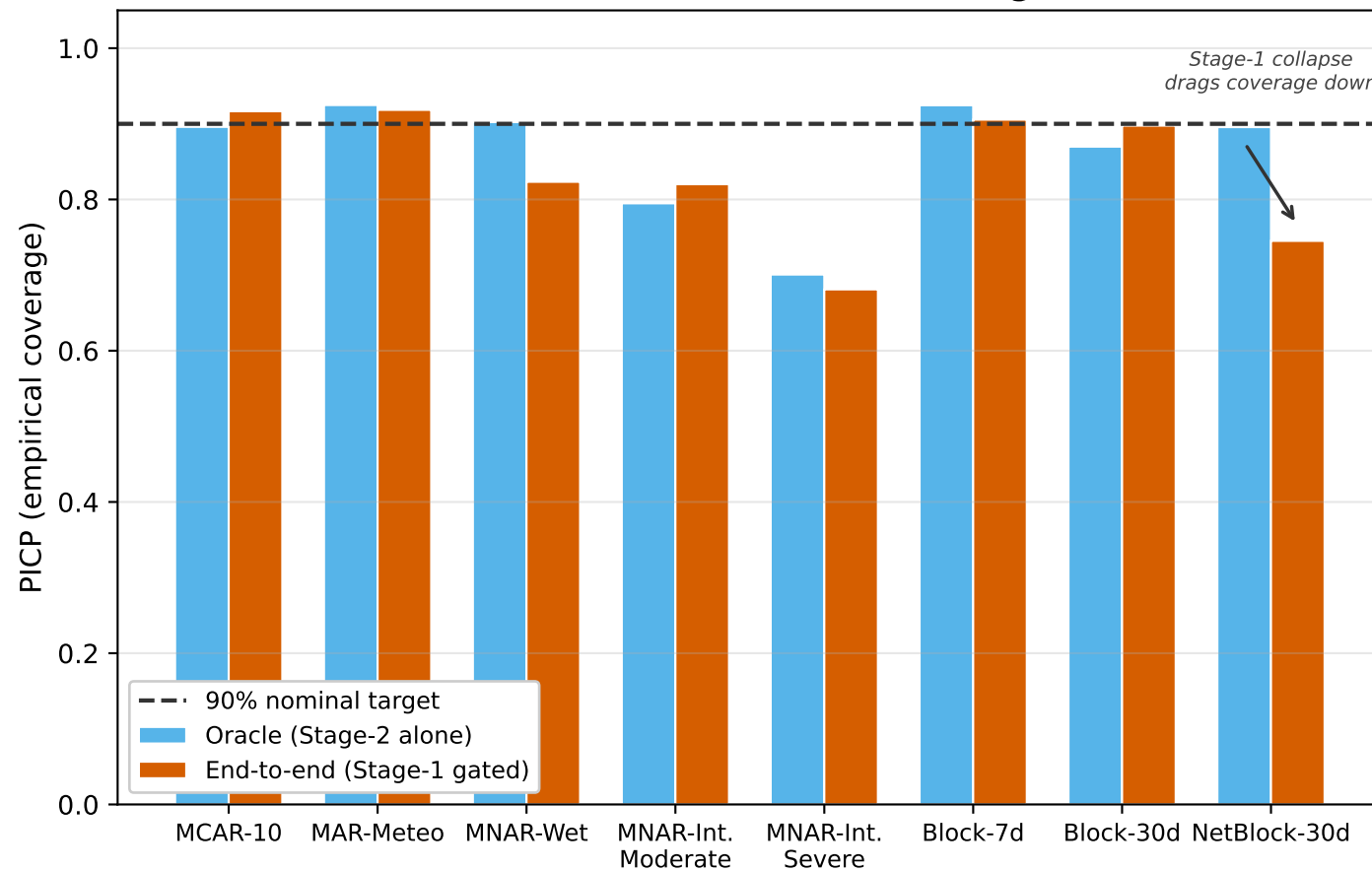
(a) Oracle vs end-to-end coverage
