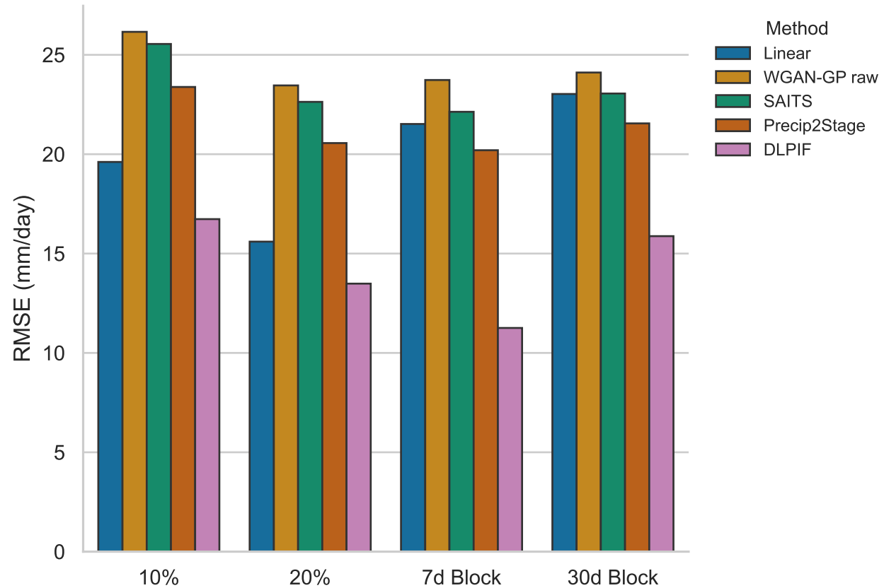
(b) Extreme Precipitation RMSE (Events \geq 95th percentile (16.74 mm/day))
