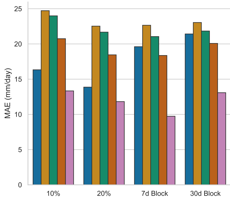
(a) Extreme Precipitation MAE (Events \geq 95th percentile (16.74 mm/day))
