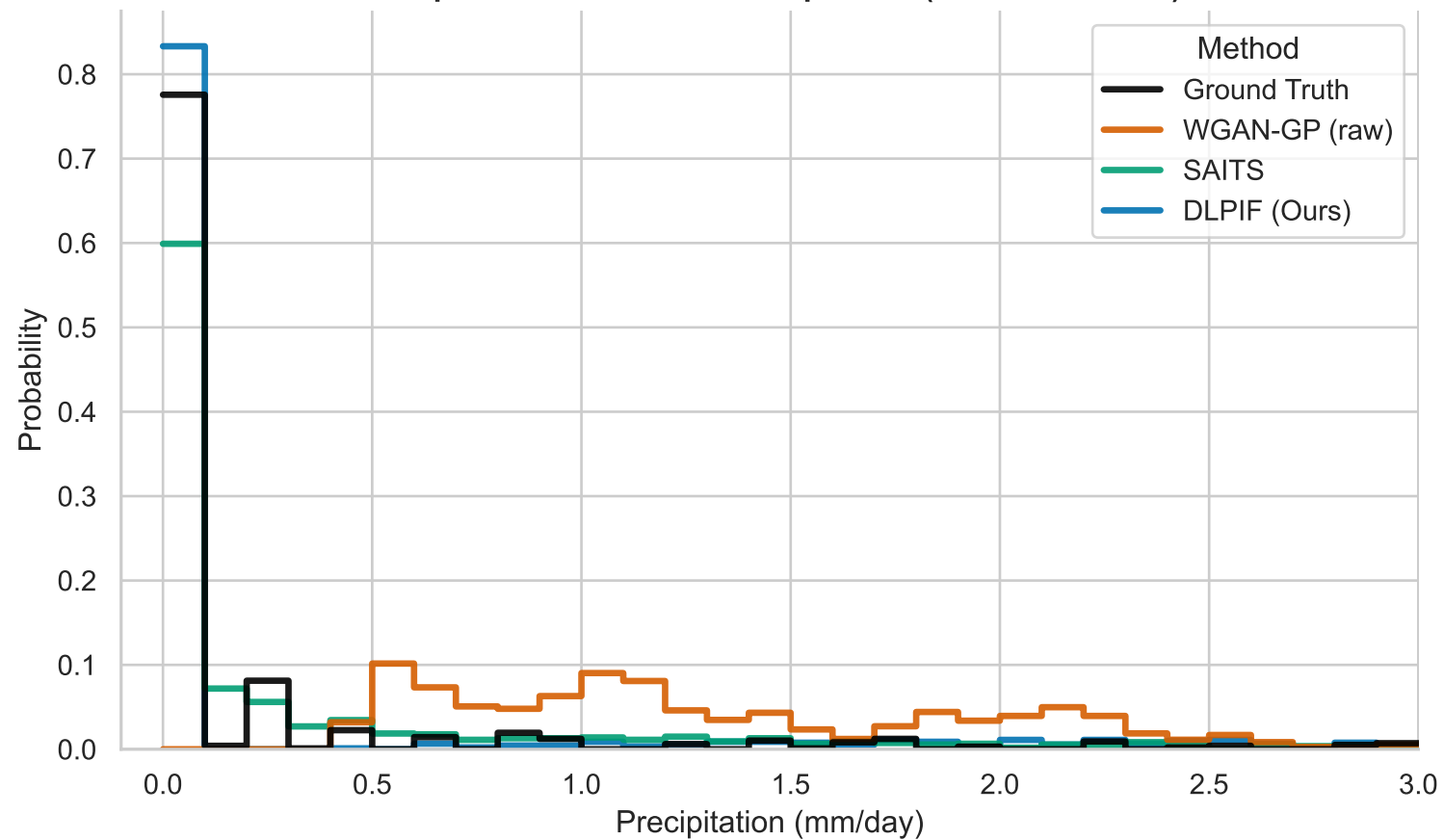
Precipitation Distribution Comparison (Near-Zero Zoom)
