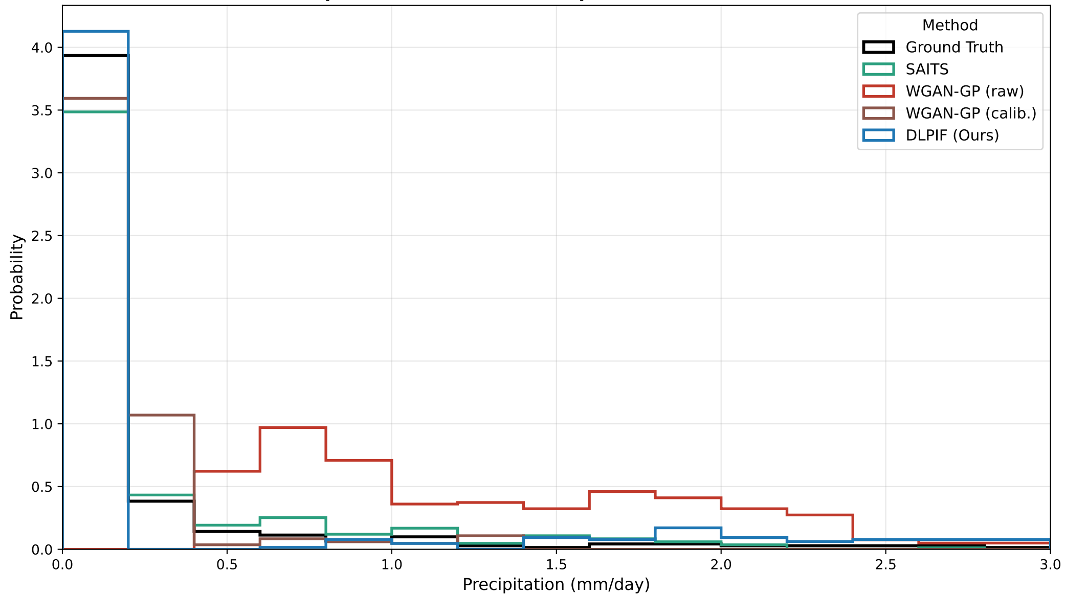
Precipitation Distribution Comparison (Near-Zero Zoom)
