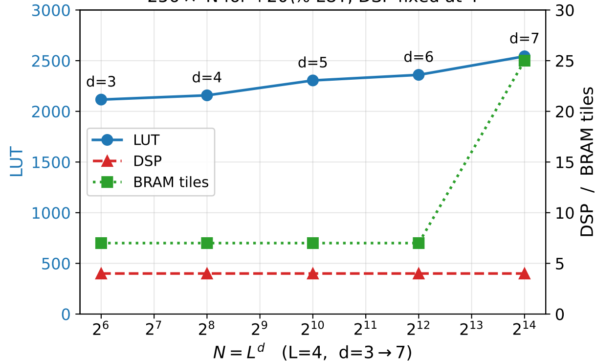
Fixed-width compute as depth grows (L=4): 256 × N for +20\% LUT, DSP fixed at 4
