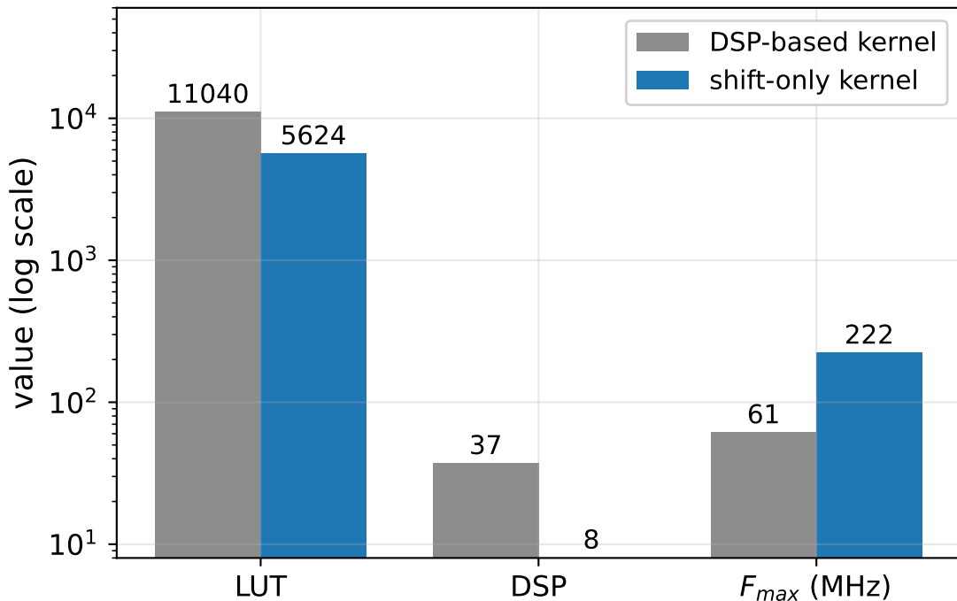
Shift-only vs DSP-based 8-pt sub-NTT (N=4096): −49% LUT, −78% DSP, 3.6 \times F_{max}
