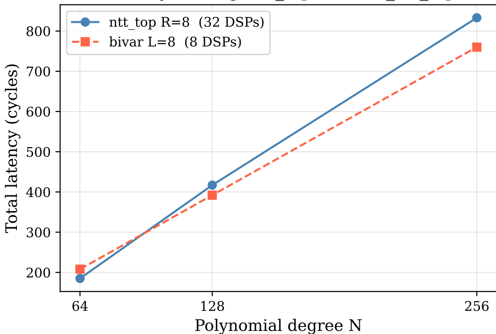
Latency Scaling: ntt_top vs bivar_ntt_top
