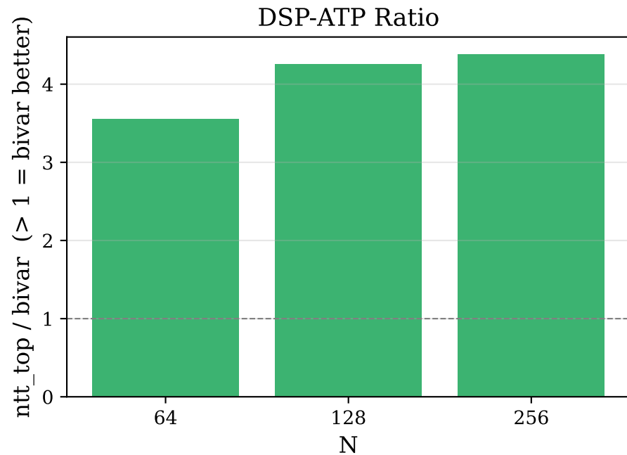
DSP Area-Time Product: ntt_top (R=8) vs bivar_ntt_top (L=8)
