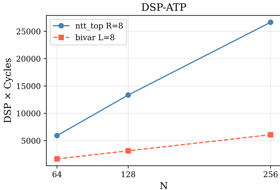
DSP Area-Time Product: ntt_top (R=8) vs bivar_ntt_top (L=8)
