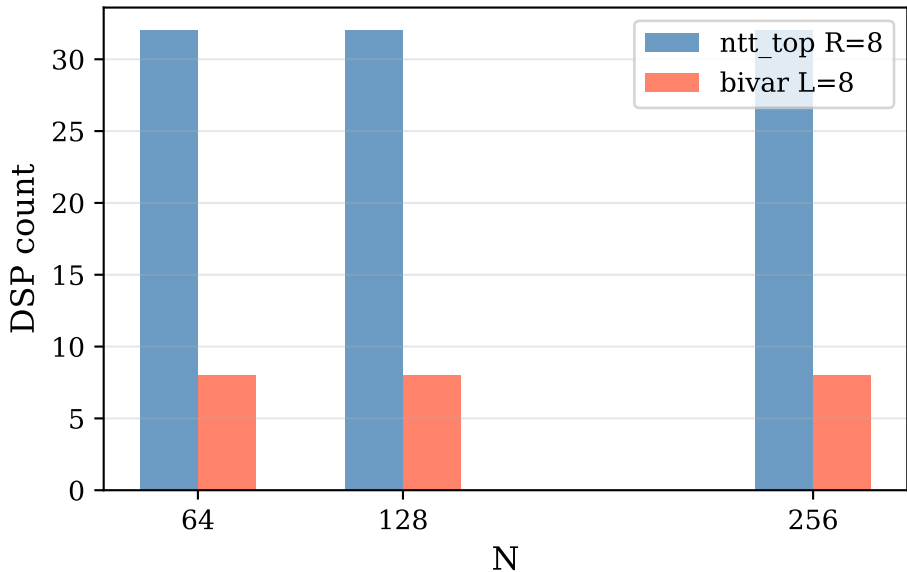
DSP Utilization vs N
