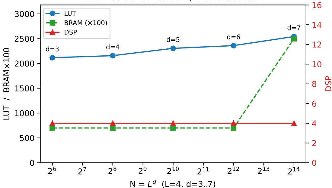
Constant compute hardware as depth d grows ( L=4 ) 256 \times N for +20% LUT; DSP fixed at 4
