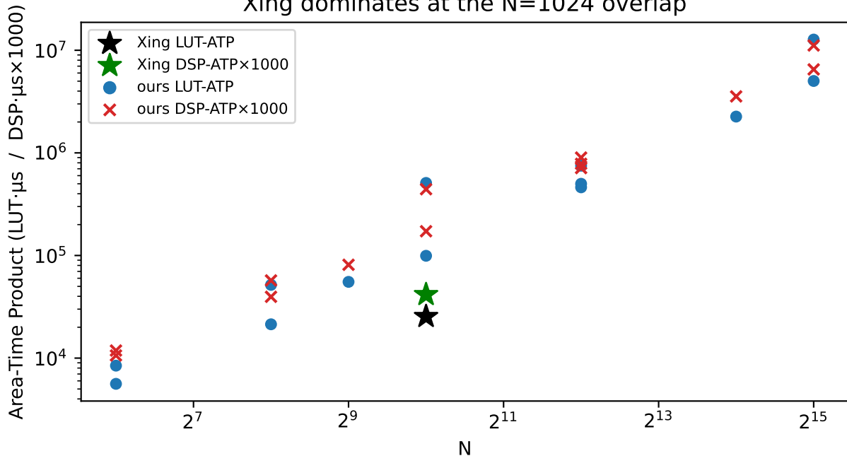
Area-time product vs N (lower is better) Xing dominates at the N=1024 overlap
