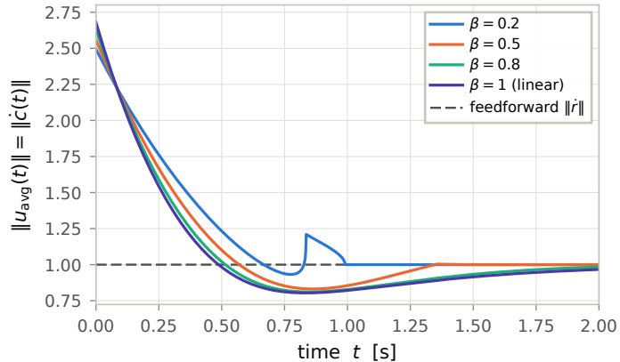
(b) averaged control effort
