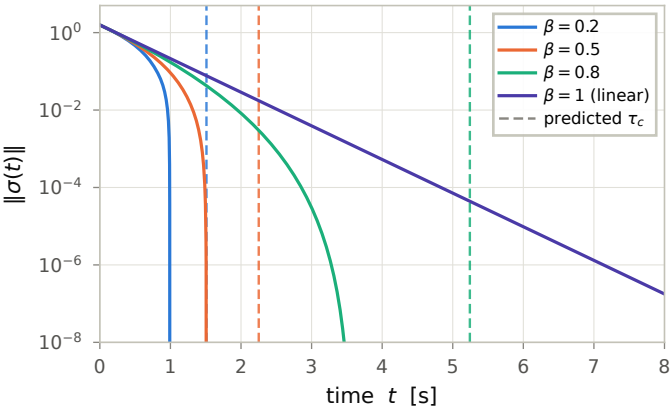
(a) finite-time arrival vs. bound \tau_c
