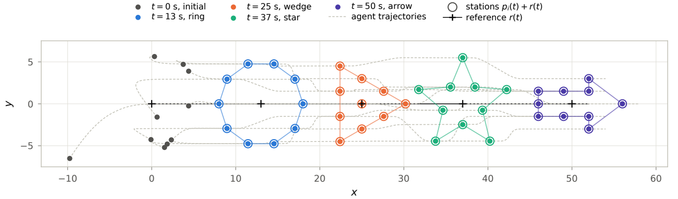
Fig. 2. Trajectory profiles for a swarm of n = 10 agents tracking a linear reference r(t) = [t, 0]^\top while reconfiguring across four distinct centered templates: ring, wedge, star, and arrow. Dashed curves represent individual agent paths; hollow circles mark the time-varying target stations p_i(t) + r(t) over template outlines, and filled dots indicate instant agent positions. Minimum-jerk blends over 4 s intervals preserve the centering condition \sum p_i = 0 throughout transitions, with agent-to-station slot assignment optimized via the Hungarian algorithm. A video of this simulation is available as drive link .
