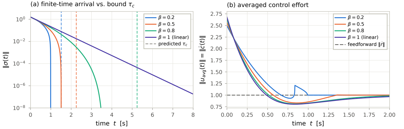
Fig. 1. Performance of the centroid channel across sliding exponents \beta \in \{0.2, 0.5, 0.8\} alongside the linear baseline \beta = 1 . (a) Convergence of the centroid tracking error \|\sigma(t)\| plotted against the analytical settling-time bounds \tau_c Eq. (4) (dashed lines). (b) Averaged control effort \|u_{avg}(t)\| = \|\dot{c}(t)\| decaying to the feedforward baseline \|\dot{r}\| .
