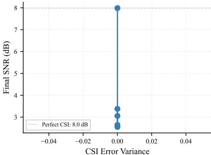
(a) SNR vs. CSI Error
