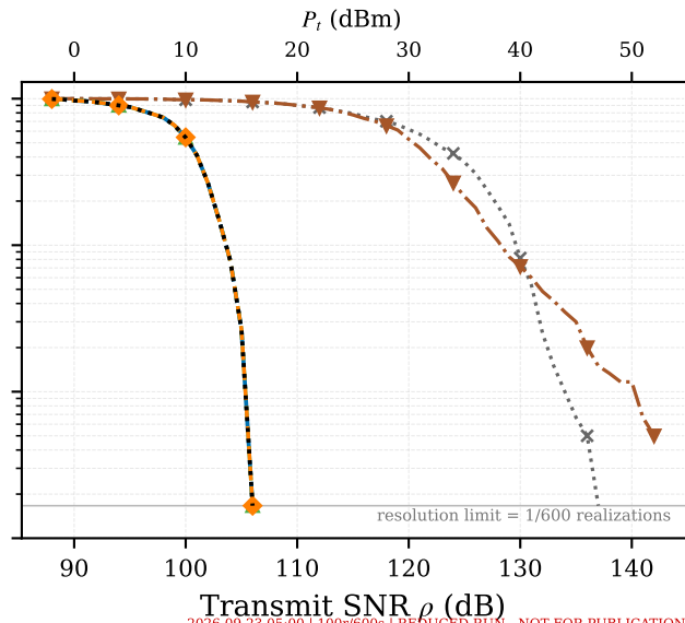
(b) R_{th} = 2 bit/s/Hz
