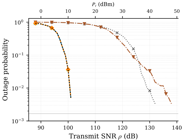
(a) R_{th} = 1 bit/s/Hz
