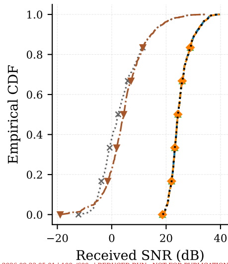
(c) SNR distribution, full surface
