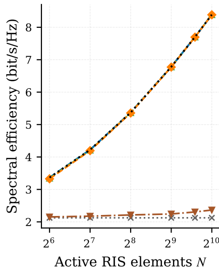
(b) Rate vs surface size
