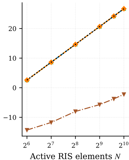
(a) Array-gain scaling
