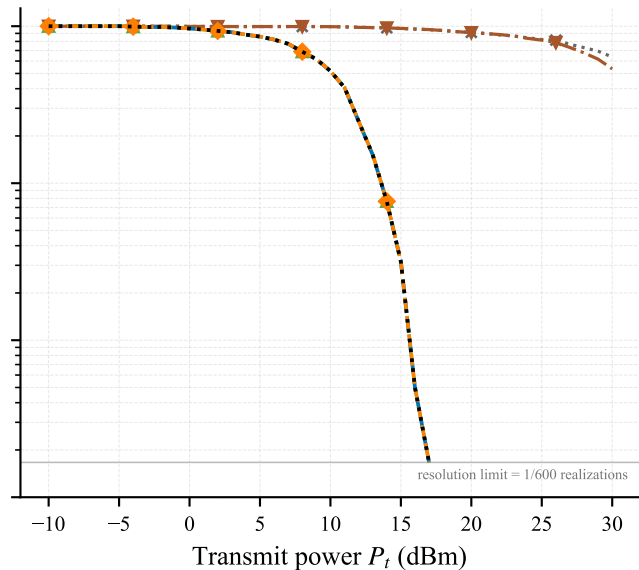
(b) R_{th} = 2 bit/s/Hz
