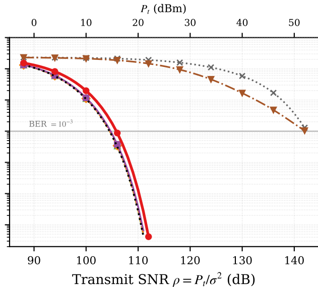
(b) 16QAM
