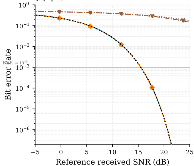
(a) QPSK
