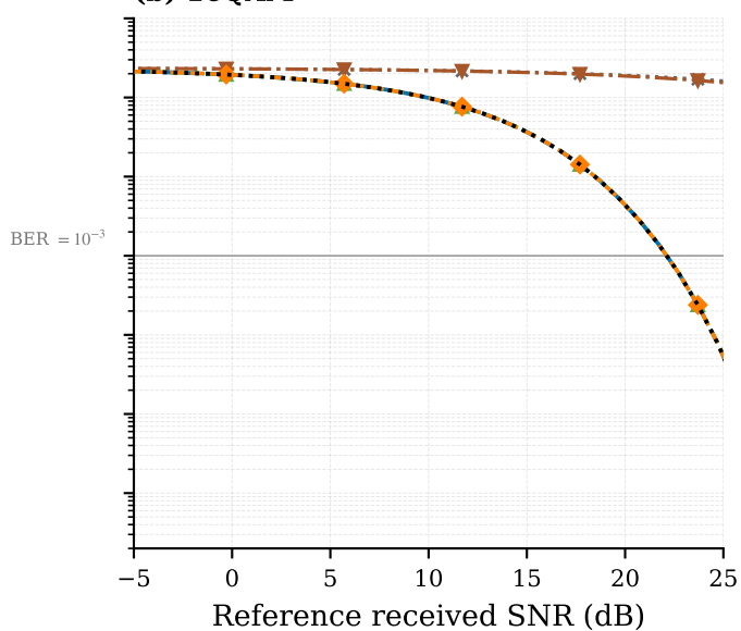
(b) 16QAM
