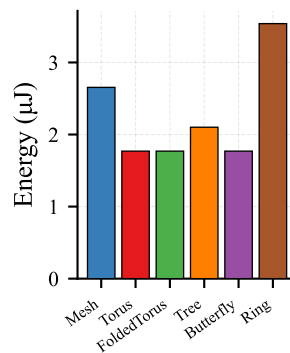
(b) Total Energy
