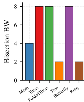
(e) Bisection Bandwidth
