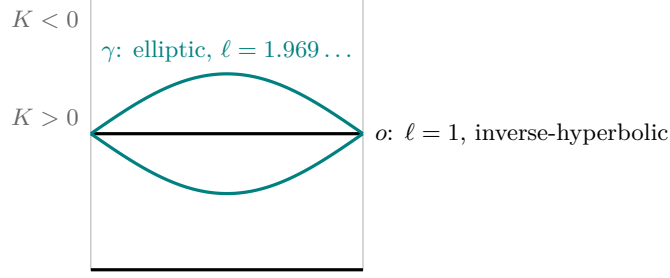
FIGURE 1. Schematic of Theorem 1.13 on the fundamental domain [0, 1] \times [-\frac{1}{2}, \frac{1}{2}] , sides identified. The two teal strands form a prime geodesic string \gamma of class 2\beta_0 : it winds twice in x while oscillating once about o , born of o at a period doubling. Lengths are with respect to g_\epsilon at \epsilon = 5/\pi^2 , where numerically \gamma is the only prime string of its class (Remark 12.2); the picture is topological.
