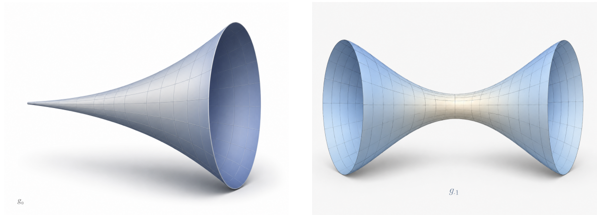
FIGURE 1. Schematic renderings of the two warped products. On the left, g_0 = dx^2 + e^{2x} d\theta^2 , with no class \beta geodesic. On the right, g_1 = dx^2 + \cosh^2(x) d\theta^2 , with a unique class \beta geodesic at the waist x = 0 .
