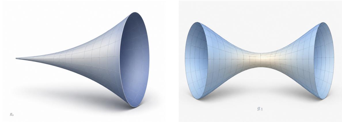
FIGURE 1. Schematic renderings of the two warped products. On the left, g_0 = dx^2 + e^{2x} d\theta^2 , with no class \beta geodesic. On the right, g_1 = dx^2 + \cosh^2(x) d\theta^2 , with a unique class \beta geodesic at the waist x = 0 .
