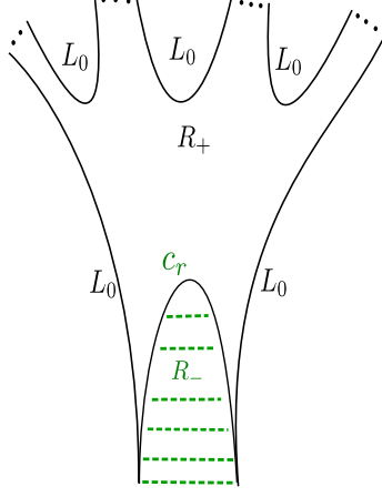
FIGURE 1. The labels L_0 indicate that the Lagrangian subbundle is constant with corresponding fiber L_0 . The curve c_r bounds R_- .
