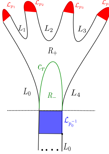
FIGURE 2. Over the boundary components with black labels L_i the Lagrangian subbundle \mathcal{L}_r^n is constant with corresponding fiber L_i . Over the i 'th red boundary component the Lagrangian subbundle corresponds to the path of Lagrangians p_i . Likewise over the right boundary component of the blue region, the Lagrangian subbundle corresponds to the path of Lagrangians p_0^{-1} . In the red striped regions we have removed the curvature of the connection, in the blue striped region we have added it.
