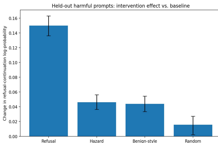
Figure 2. The refusal direction produces a larger raw shift in refusal-continuation likelihood than the control interventions on held-out harmful prompts.
