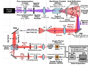
Figure 1: Schematic representation of the spontaneous parametric down-conversion setup.
