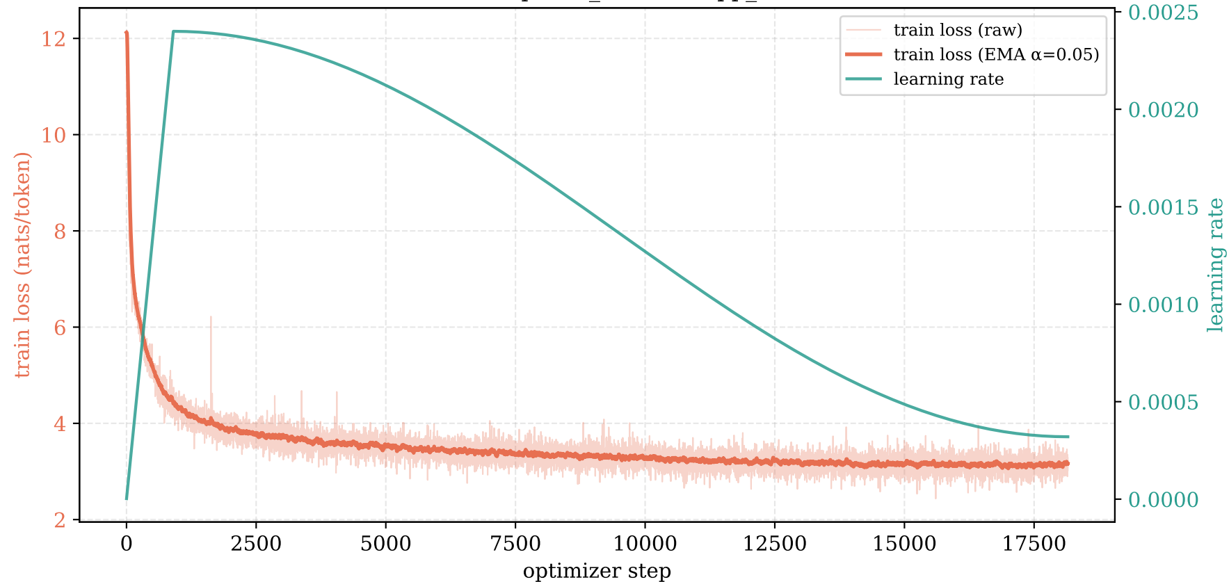
Qwen3-0.6B FAITHFUL — train loss & cosine LR (COMPLETE run, 18,150 steps / 1.19B tok)
