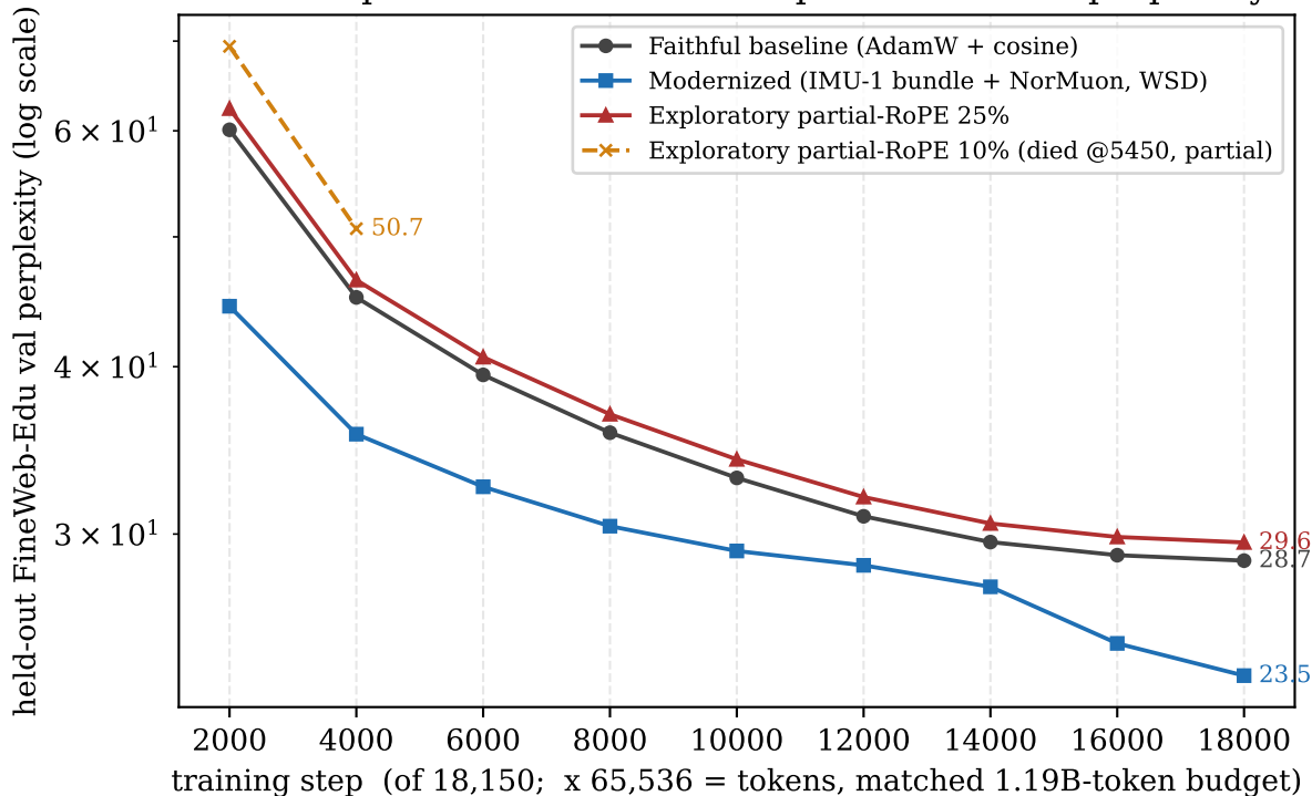
Three-build comparison at matched compute: validation perplexity vs s
