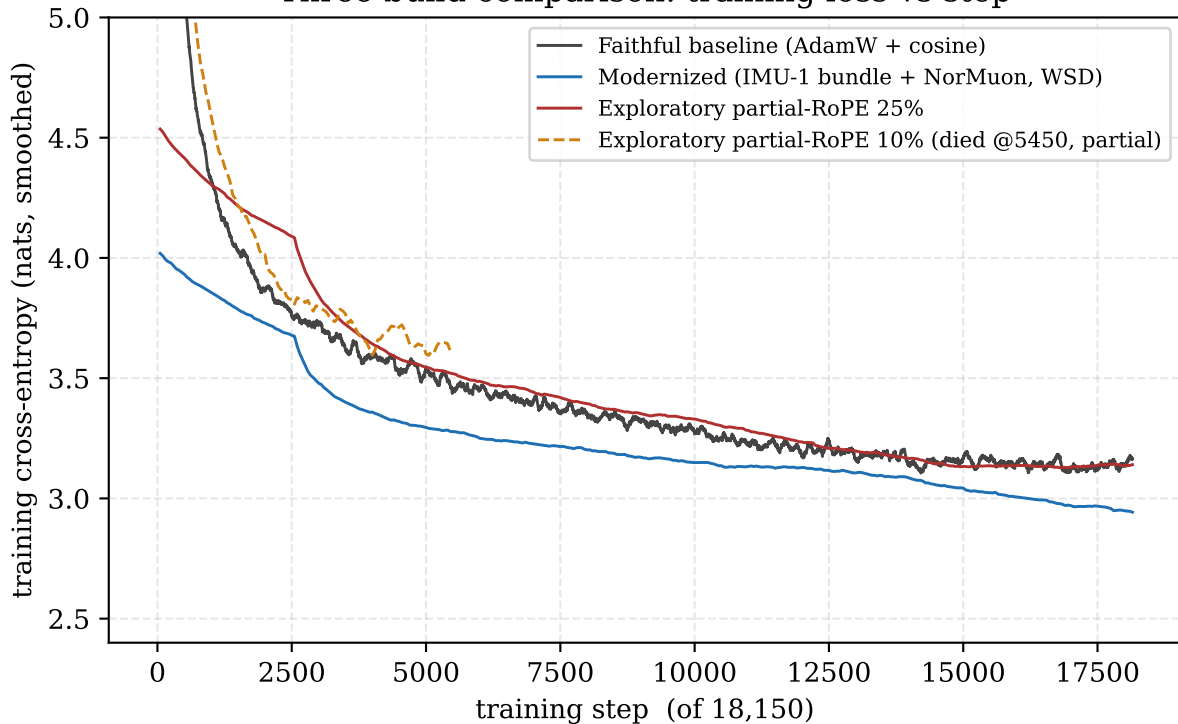
Three-build comparison: training loss vs step
