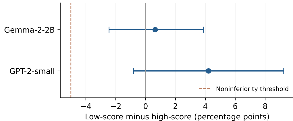
Positive-sentiment probability
