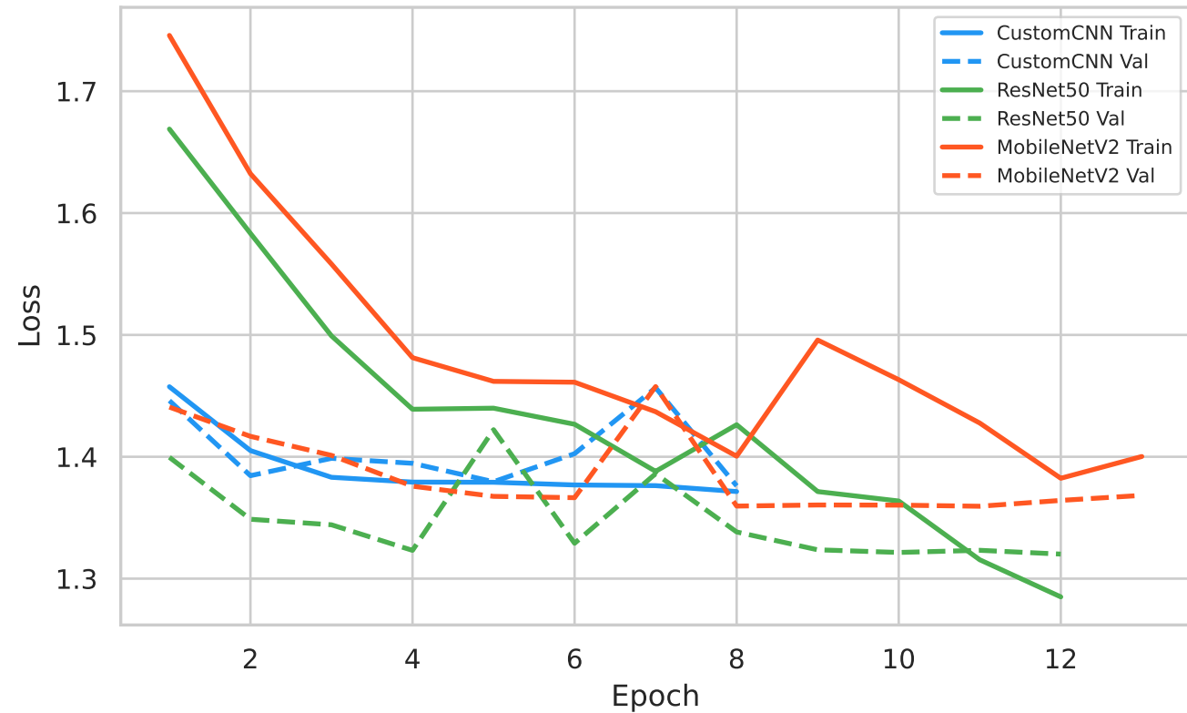
Training & Validation Loss
