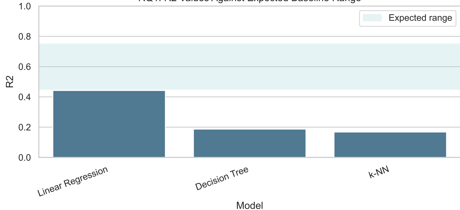
RQ1: R2 Values Against Expected Baseline Range
