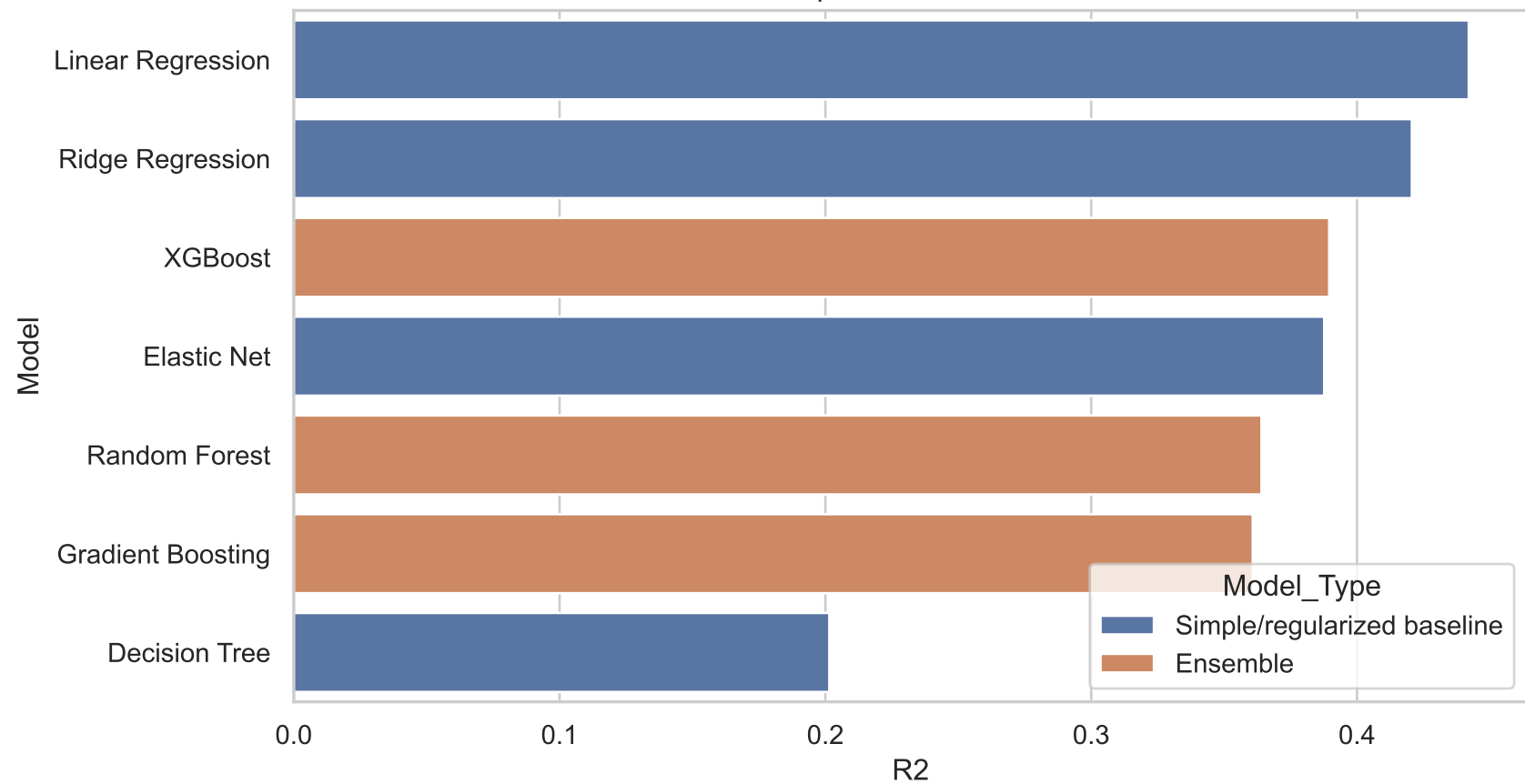
RQ2: R2 Comparison of Candidate Models
