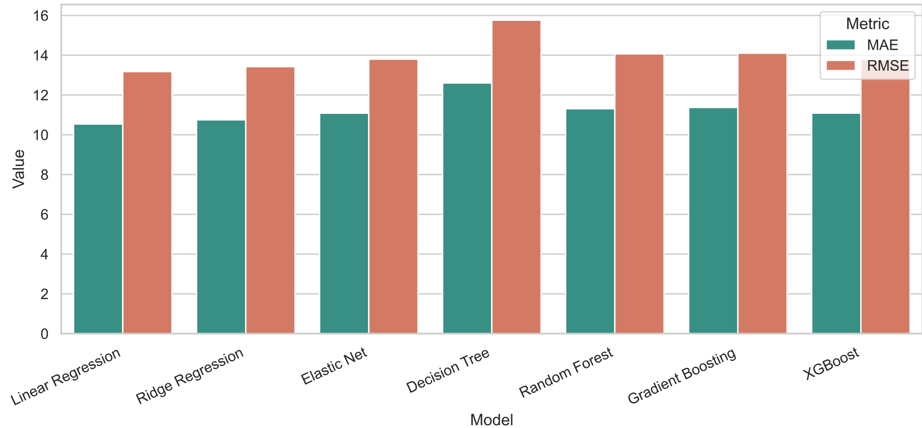
RQ2: Candidate Model Error Metrics
