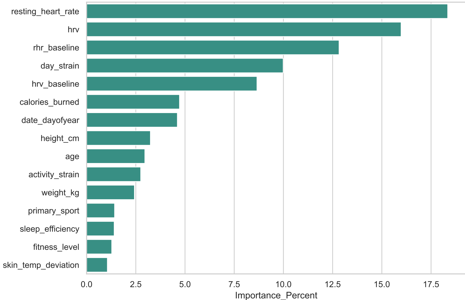
RQ4: Top Aggregated Feature Importances
