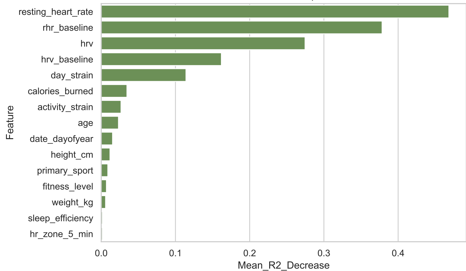
RQ4: Permutation Importance
