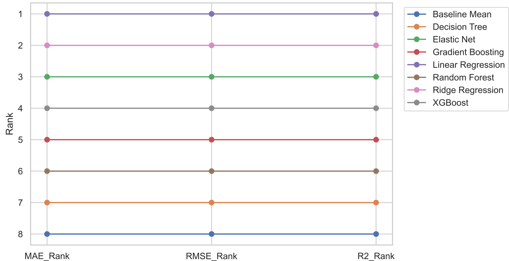
RQ5: Ranking Bump Chart
