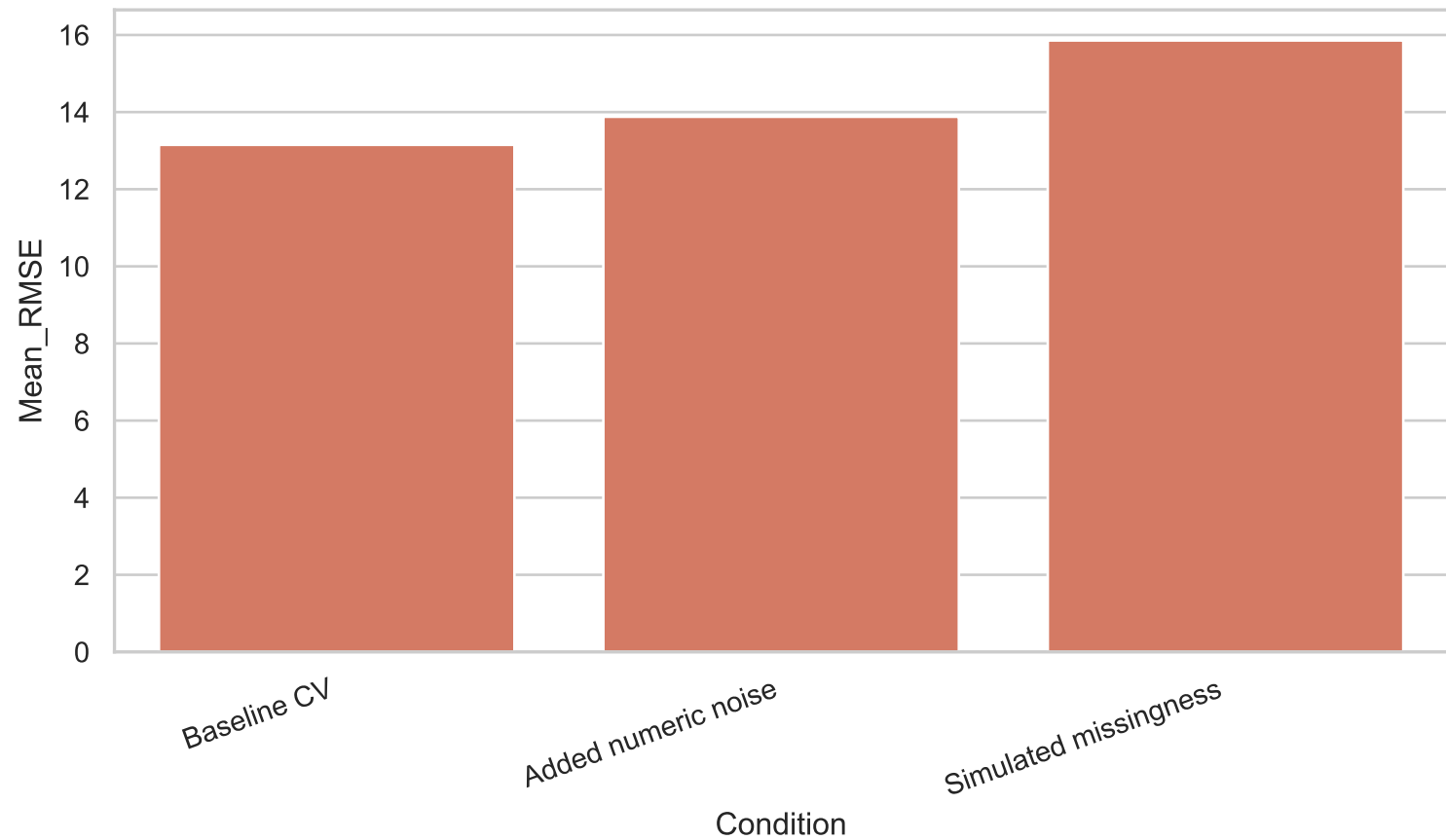
RQ6: RMSE Robustness
