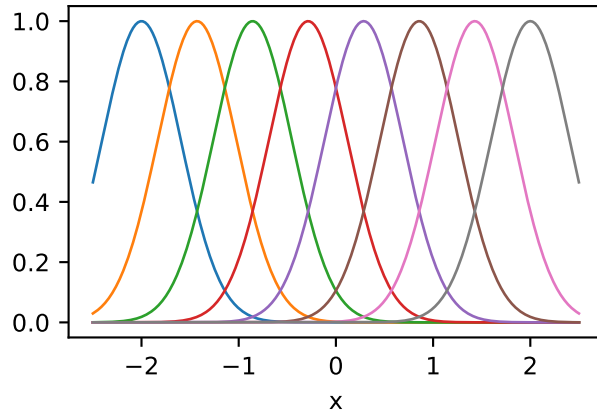
Gaussian RBF basis
