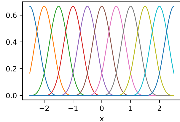
Cubic B-spline basis
