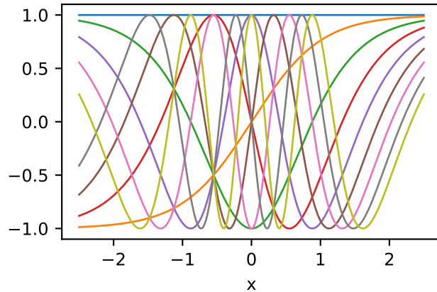
Chebyshev basis (tanh input)
