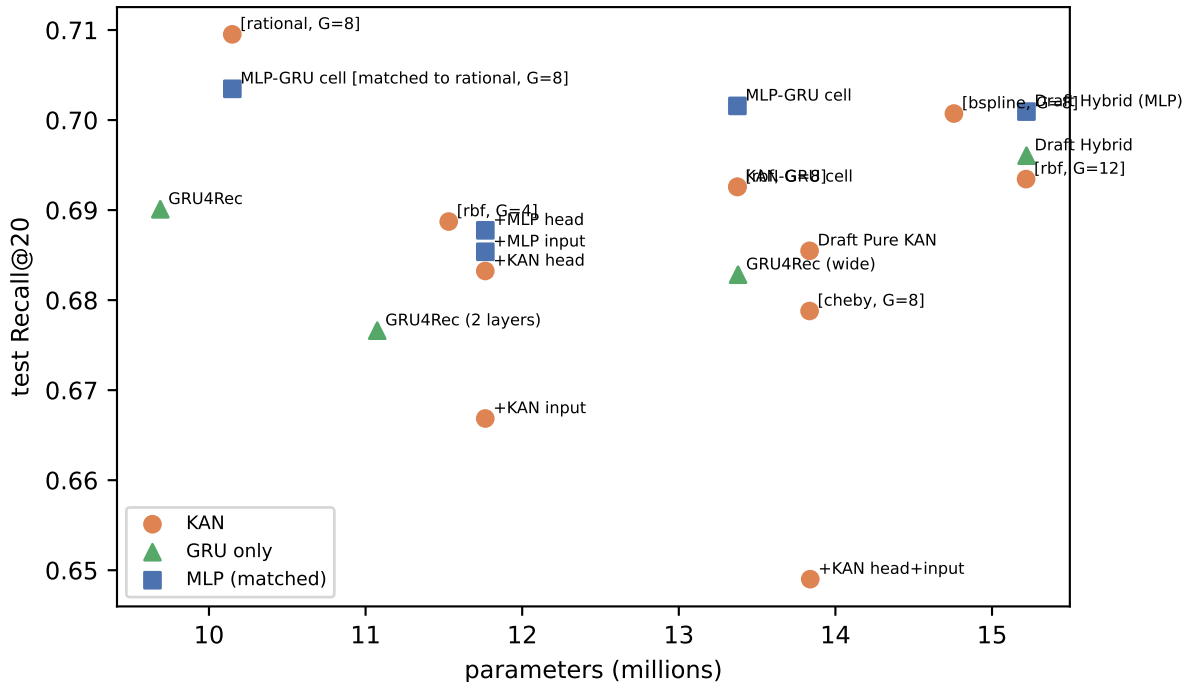
Accuracy vs model size, YooChoose 1/64
