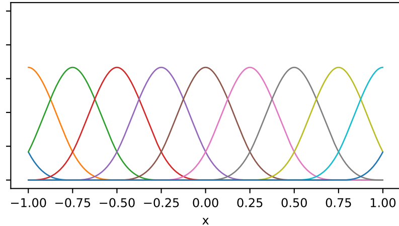
Correct cubic B-spline
