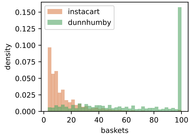
Baskets per user
