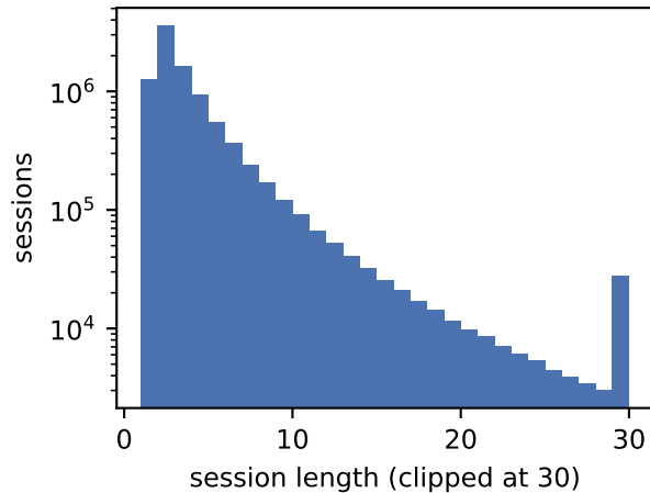
YooChoose: clicks per session (raw)
