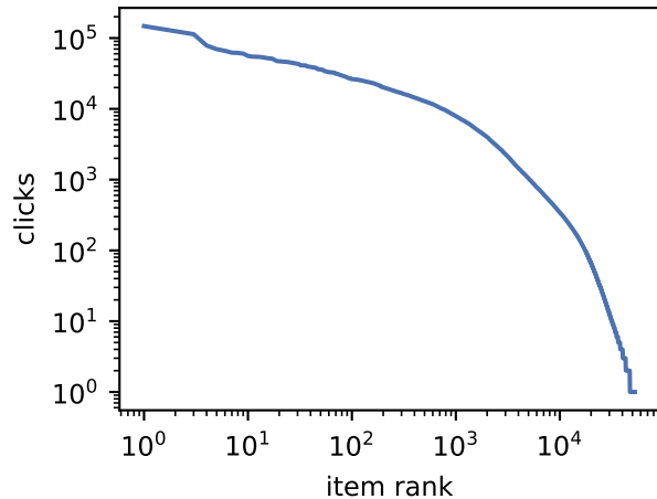
YooChoose: item popularity (raw)
