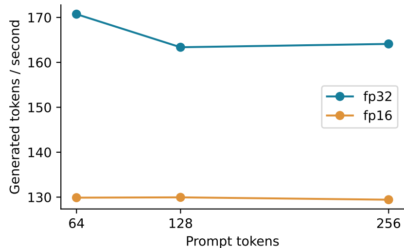
Selected adapter, batch 4, 64 new tokens
