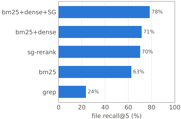
Retrieval quality spans a 3× range
