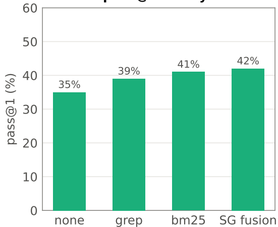
...and pass@1 barely moves
