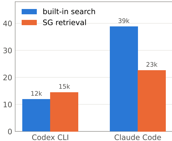
How much context the harness re-sends
