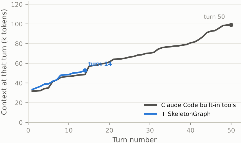
One task (Astropy): shorter AND lower context here
