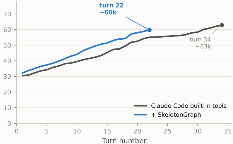
All 100 paired tasks (median): same climb, SG stops sooner
