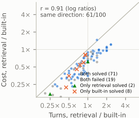
(a) Per task, cost follows turns
